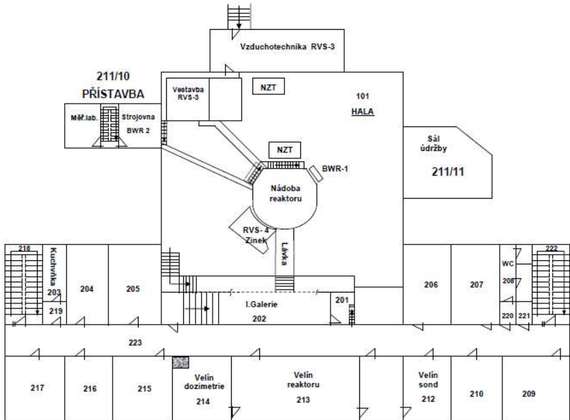
Fig. C2 LVR-15 reactor hall
