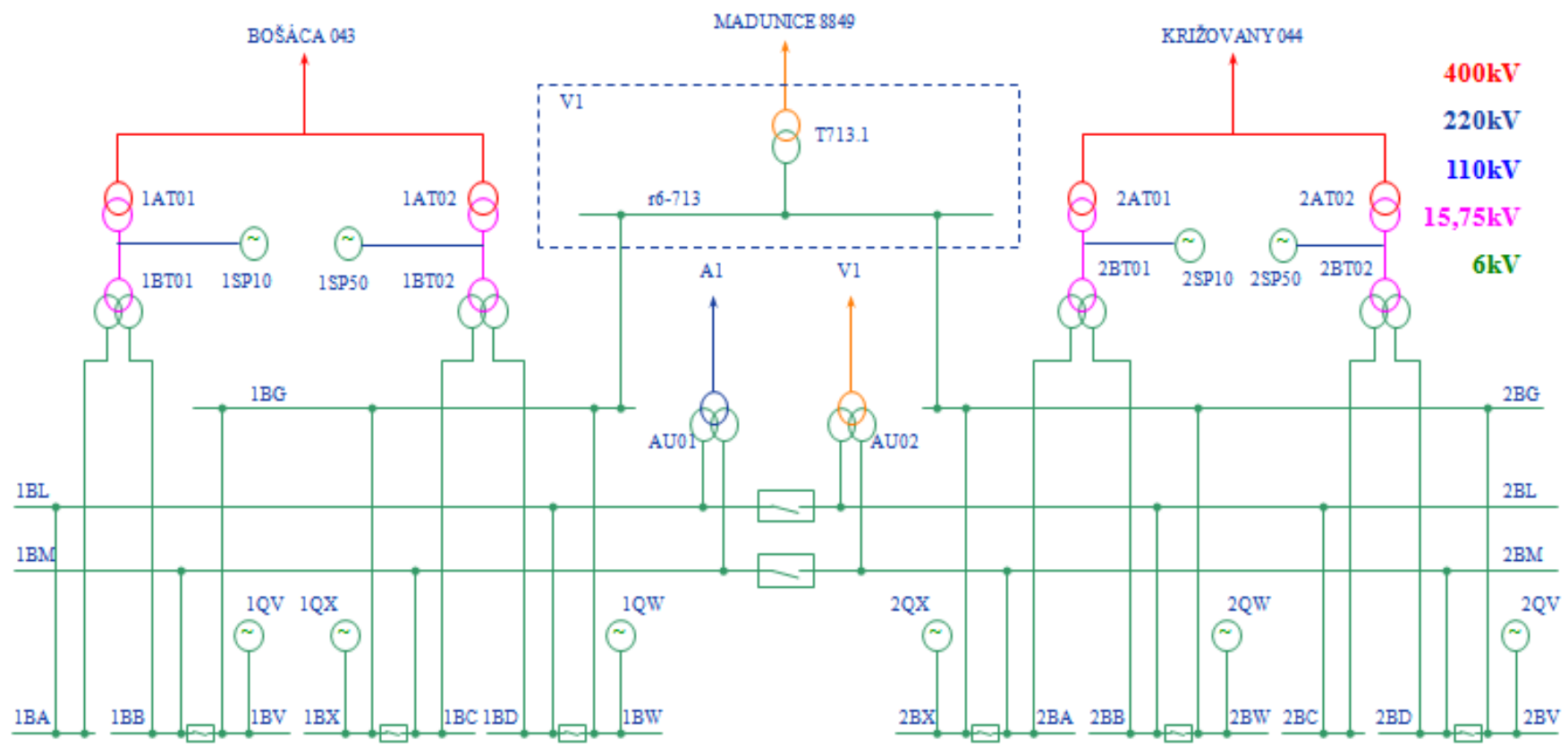
Figure 9: EBO3,4 power distribution diagram
