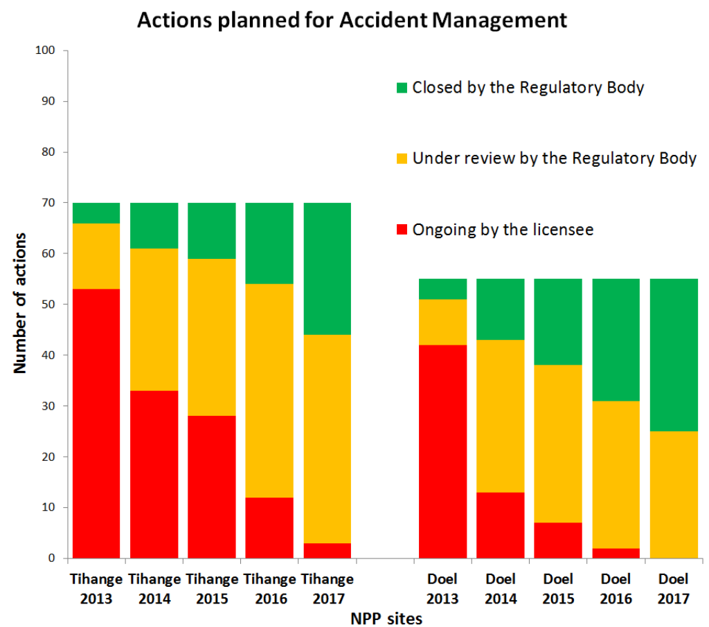
Figure 8 : Evolution of the severe accident management at Doel and Tihange since 2013.
